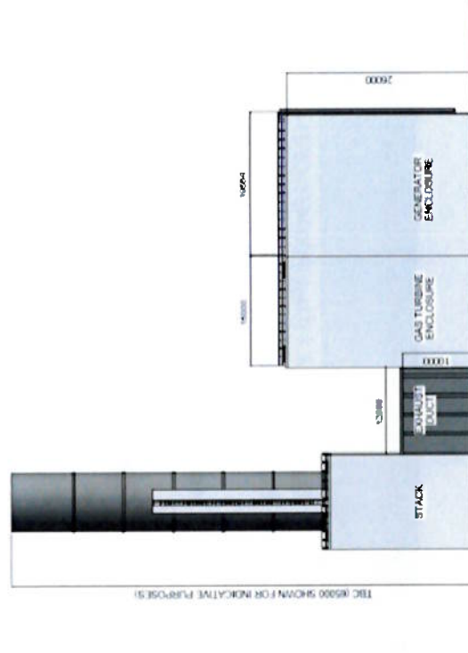
Figure 4 Proposed Elevation - East View – No SCR and/or CO Catalyst Building (Scenario 4)
